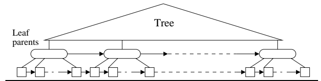
Figure 2: Internal jump-pointer array
