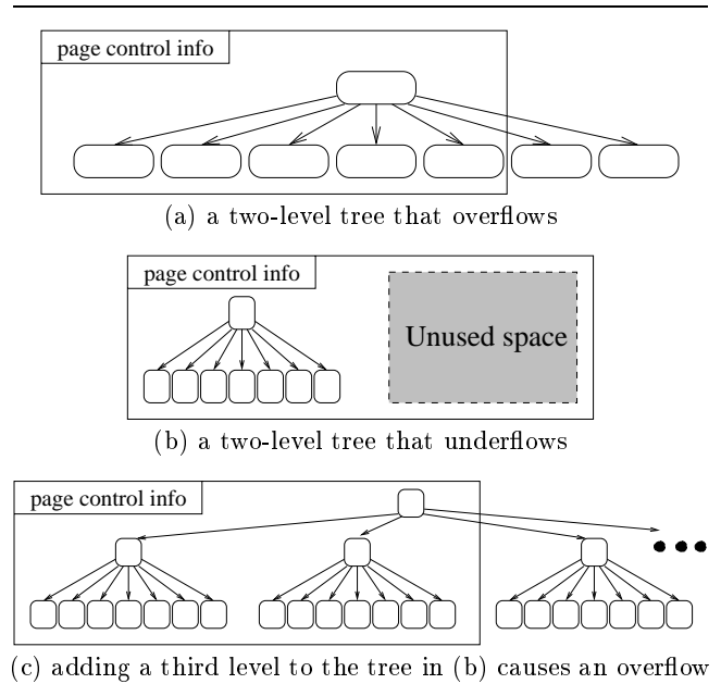
Figure 6: The node size mismatch problem
